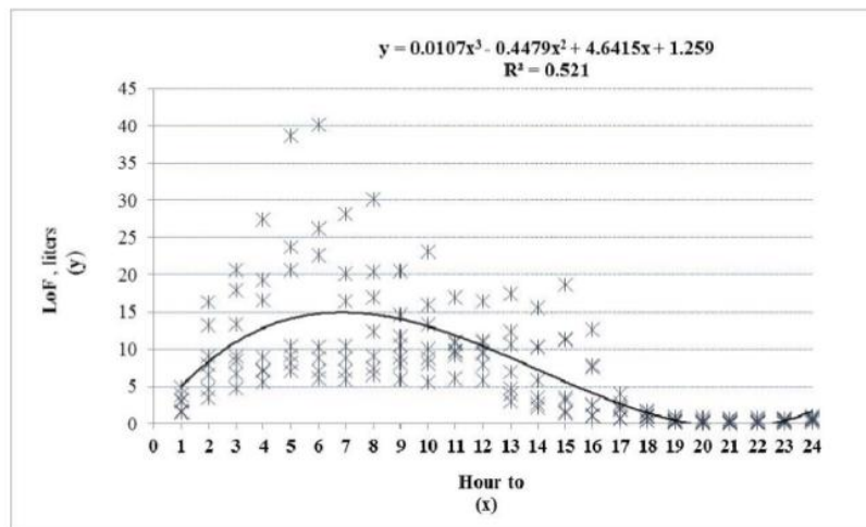
Figure 6. LoF (Y) and T (x) relationship model.
