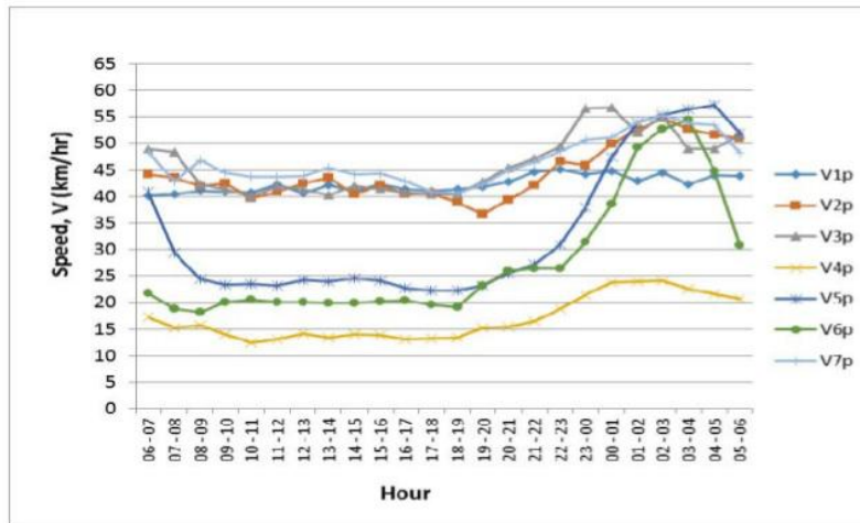
Figure 3. Vp vehicle speed fluctuations (km / hr)
